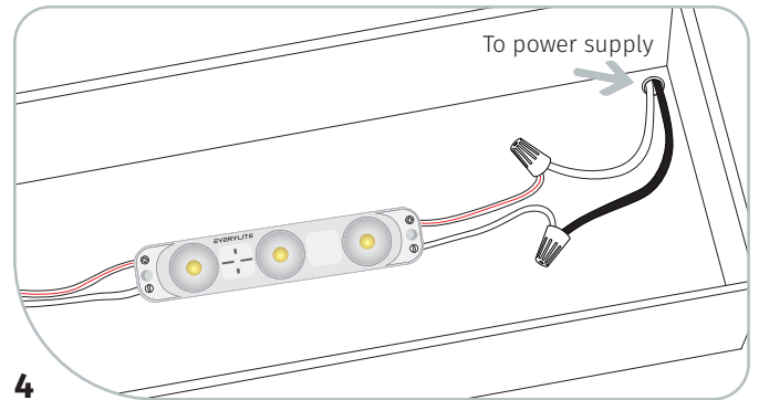
4 Connect the red striped wire (+) of the LED strip to the red wire (+) of the power supply. Connect the white wire (-) of the LED strip to the black or blue wire (-) of the power supply.
