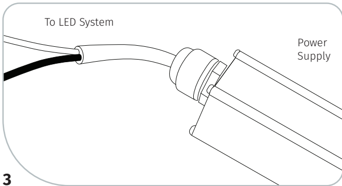
3 Run a wire from the power supply to each channel letter and connect to the first LED module on the strip.
