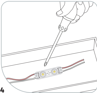
4 Use rivets, screws, or silicone to secure at least every fifth LED module within the channel letter.
